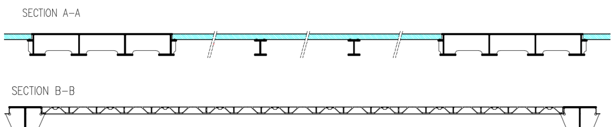
Figure 27 RAMSSES deck arrangement
