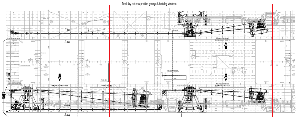
Figure 98 Deck layout of ganties and hoisting winches
