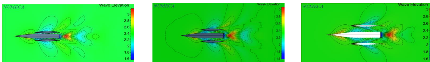
Figure 6 CFD determination of side hulls distance from centre hull
