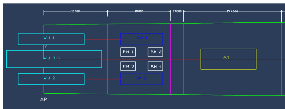
Figure 7 CODAG propulsion system with waterjets
