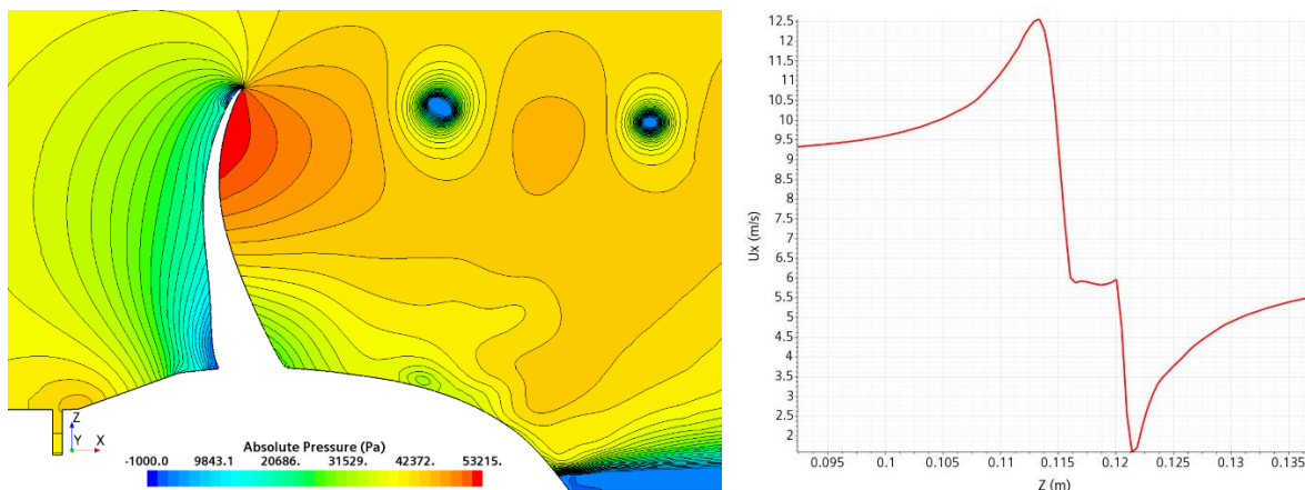
Figure 14 Contours of absolute pressure in a longitudinal section through propeller blade and hub (left) and the profile of streamwise velocity component in radial direction across tip vortex (right) from a DES-computation of flow around propeller using the finest grid with 17 million cells for a single blade.
