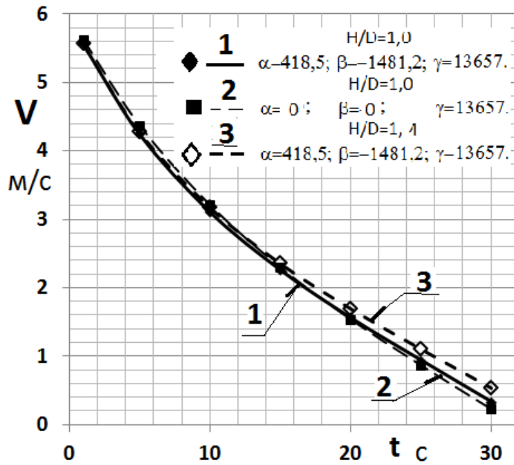
Figure 5 V_2 velocity change with time t
