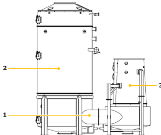
Figure 110 Example of a scrubber: 1-ducting part, 2-absorber part (outlet), 3-jet part (inlet)
