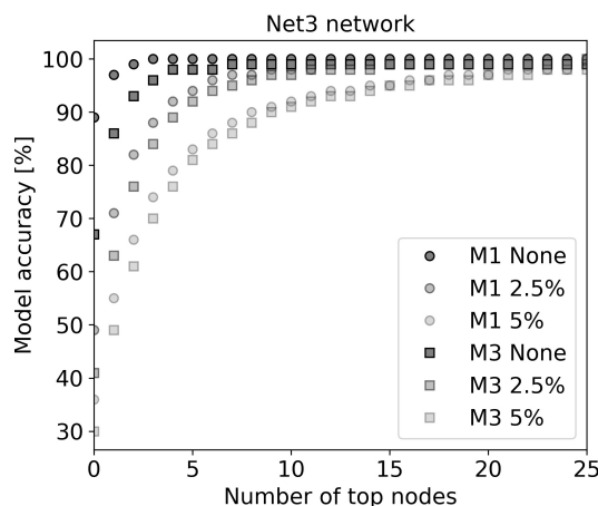
FIGURE 6. Influence of the number of top nodes on prediction model accuracy for Net3 network with 4 sensors layout and emitter coefficient range 5...15.
