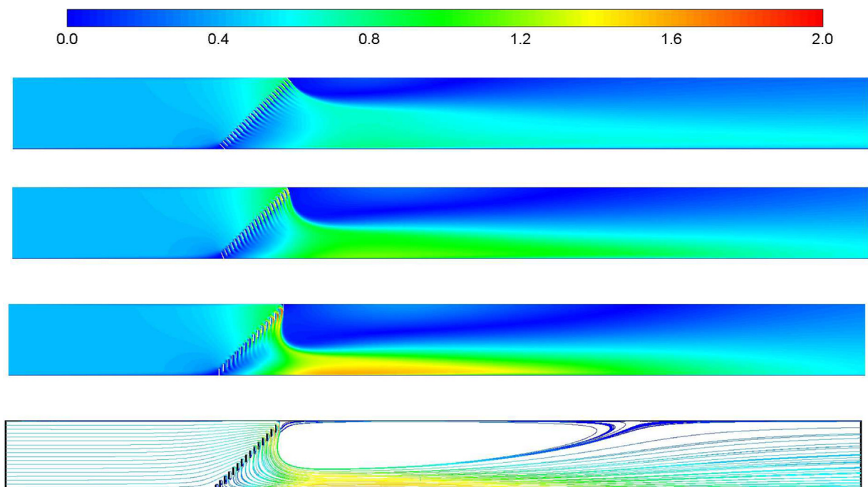
Fig. 2. Velocity magnitude (in m/s) for trash-rack configuration \alpha = 45^\circ and for \beta angles 45°, 67.5° and 90° (top to bottom) and pathlines coloured by velocity magnitude for trash-rack configuration \alpha = 45^\circ and \beta = 90^\circ .
