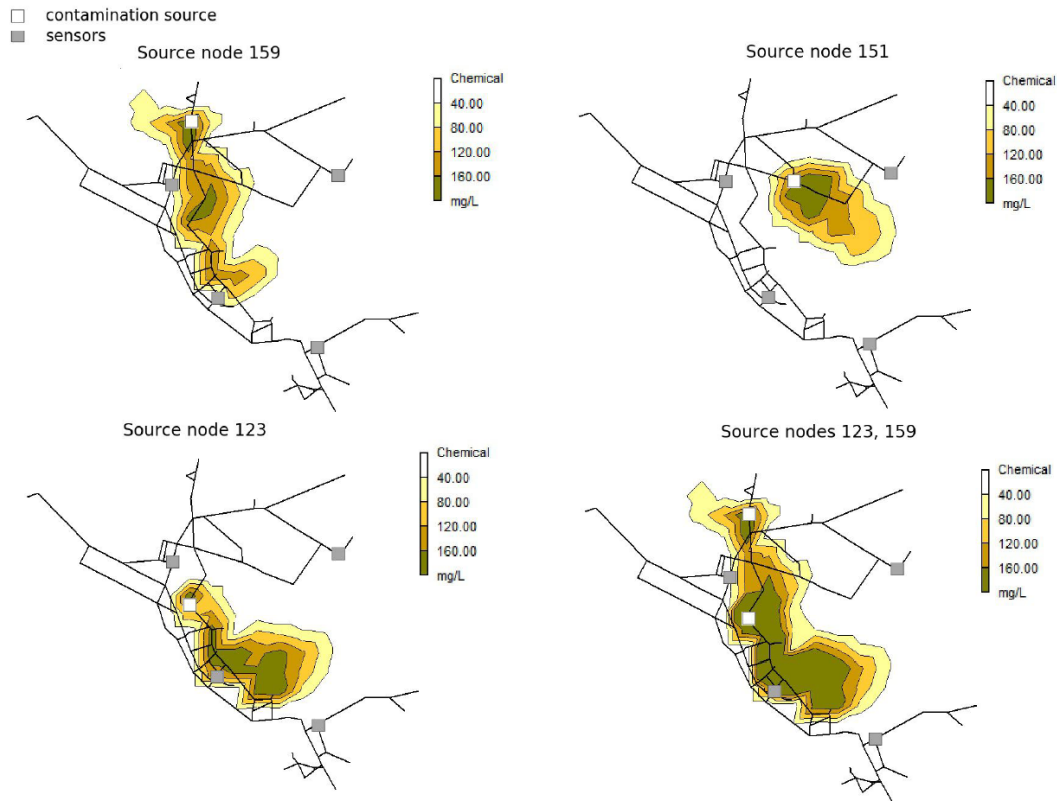
Figure 3.1: Example of single and multiple sources pollution scenarios of Net3 considered in [51].
