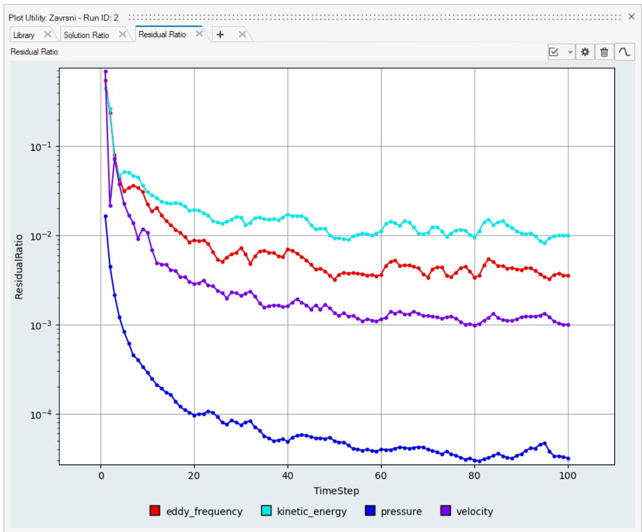
Dijagram 2. Residuali
