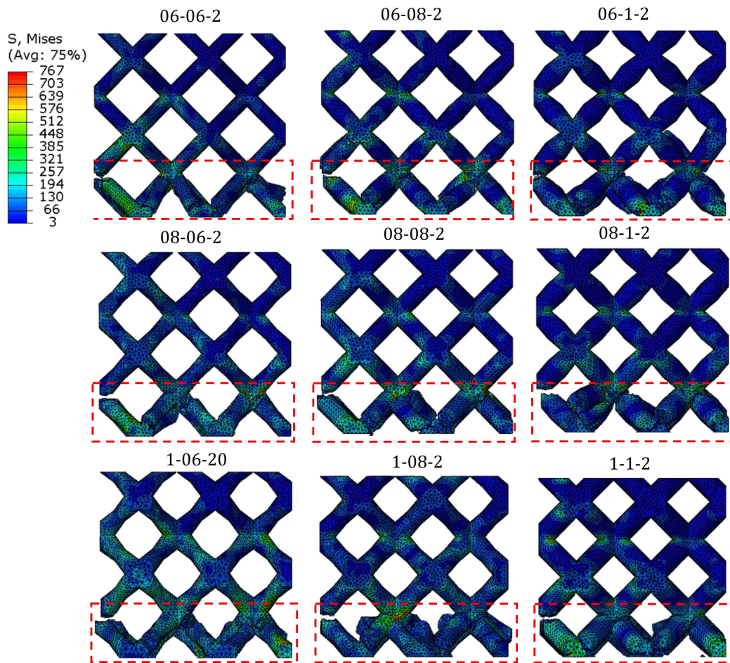
Figure 6.10: Failure of different lattice configurations with corrected effective mean d_{\text{end}} and d_{\text{mid}} diameters and 1/8 th symmetry (damaged struts are marked with red rectangle, and averaging threshold was set to the default value of 75%).
