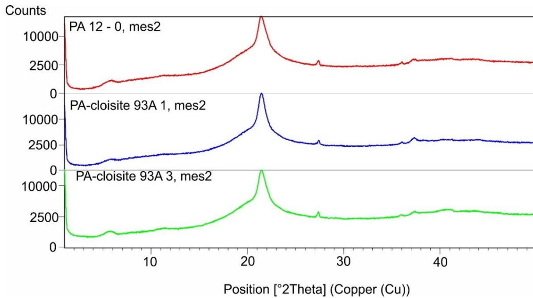
Slika 5.21 XRD dijagram za PA12, PA12/93A–1% i PA12/93A–3% [31]
