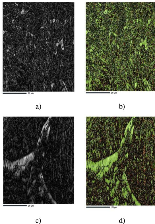
Figure 96. Results of EBSD measurements for the Cu10Al20Ag alloy: a) band contrast image, b) phase map in the as-cast state, and c) band contrast image, d) phase map in the quenched state.
