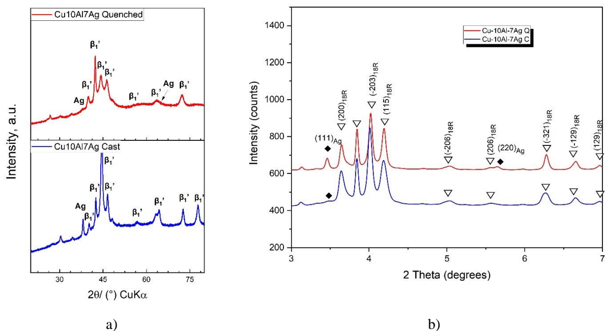
Figure 100. XRD diffractogram of Cu-10Al-7Ag SMA alloy: a) regular XRD diffractogram, b) high-energy X-ray diffraction measurements from synchrotron
