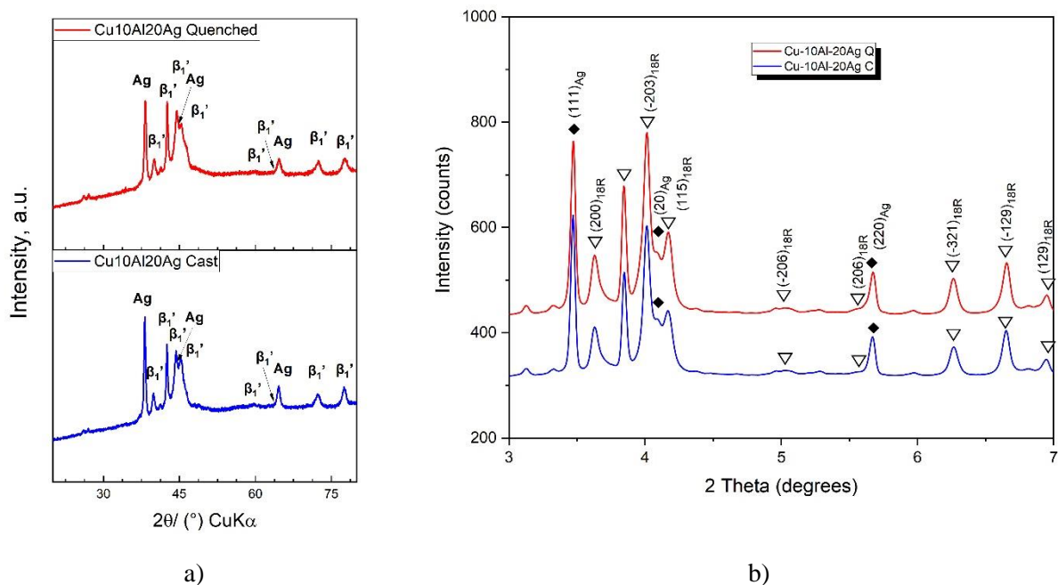
Figure 101. XRD diffractogram of Cu-10Al-20Ag SMA alloy: a) regular XRD diffractogram, b) high-energy X-ray diffraction measurements from synchrotron
