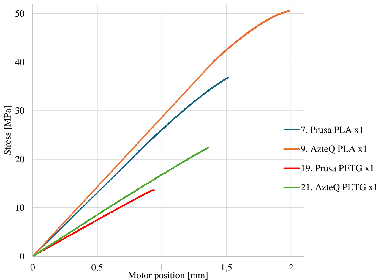
Figure 4.2. Stress–strain plot – Vertically oriented specimens
